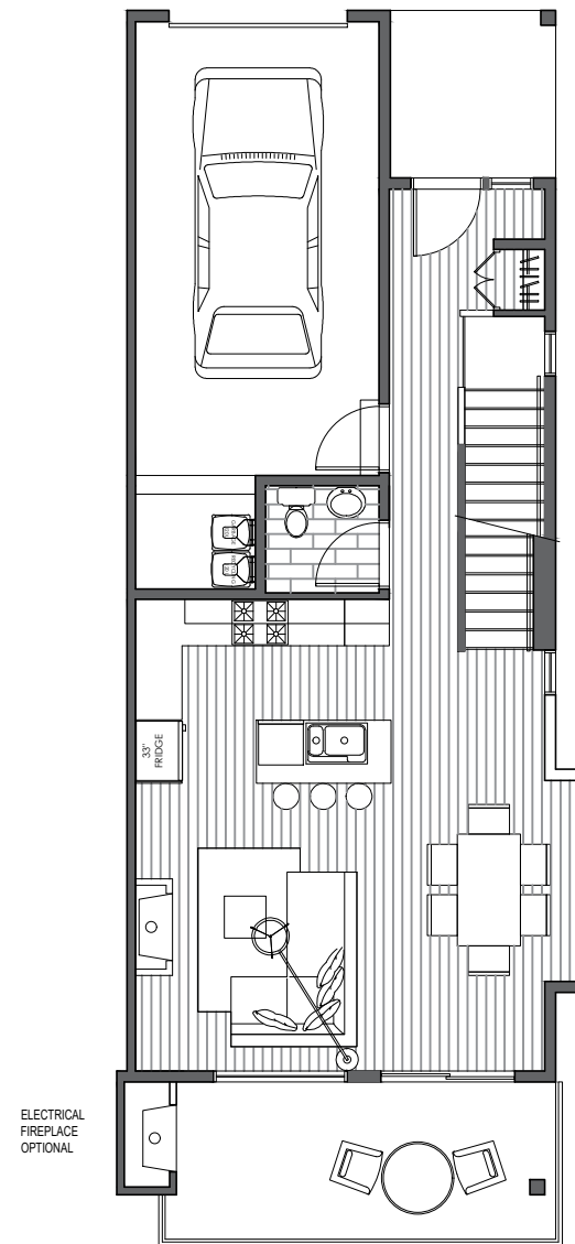
MAIN LEVEL
