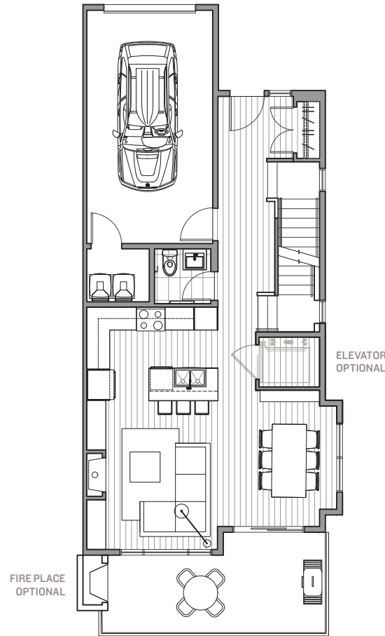
MAIN LEVEL
